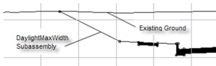
Figure 12. Daylight subassemblies use a surface target parameter to seek out and intersect surfaces based on input parameters. For example, DaylightMaxWidth Subassembly analyzes whether a cut or fill situation exists, and then uses input parameters to tie into a surface.
