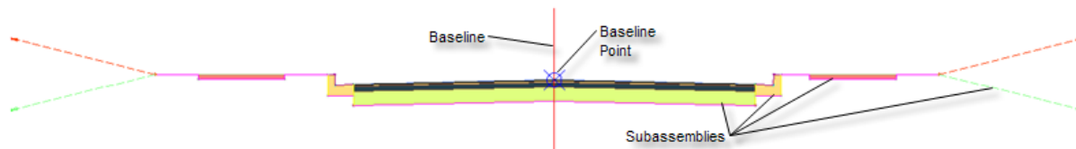
Figure 2. An assembly is made of up a combination of subassemblies such as sidewalks, curb, and lanes.
