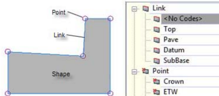
Figure 3. Subassemblies are made up of points, links and shapes. Styles can be assigned to each component, providing users with full control over display and labeling characteristics of the subassembly.
