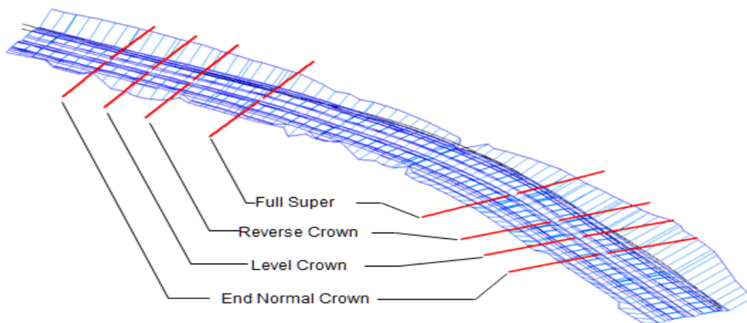
Figure 17. An example of superelevation being applied to a divided highway.
