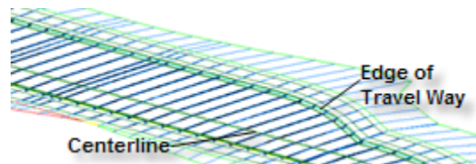
Figure 15. Specific subassemblies can use alignments, profiles, polylines, feature lines, or survey figures as targets to control the shape of the corridor.
