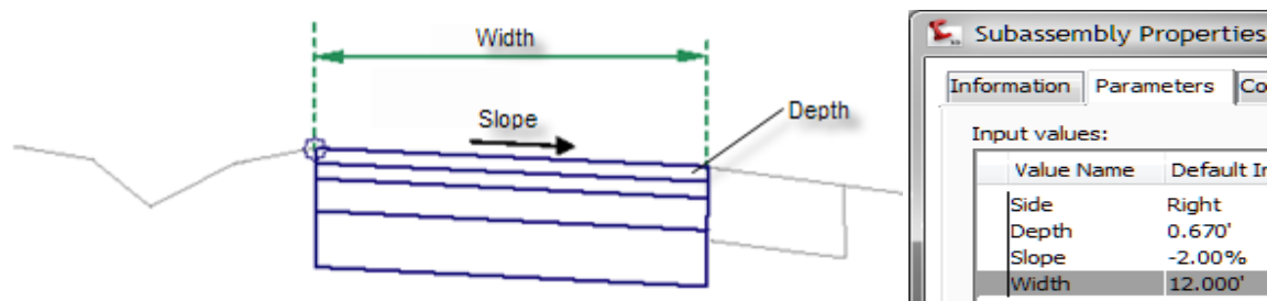
Figure 4. Input parameters allow specific components within subassemblies to be customized to fit specific project requirements. The example shown will create a lane 12' wide with a cross slope of 2% and a material course depth of 0.67 feet for the duration of the road.
