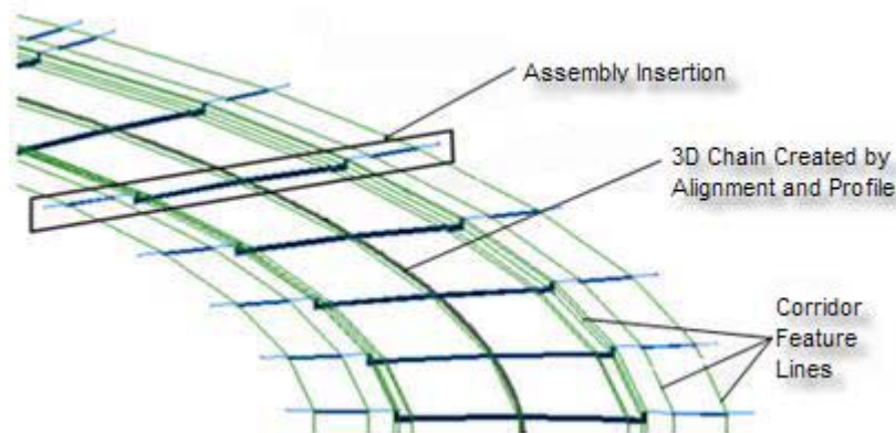
Figure 1. A 3D Chain represents an alignment and profile which control the horizontal and vertical aspects of the road. An assembly is then inserted along this path at user-defined increments and is connected longitudinally by corridor feature lines.
