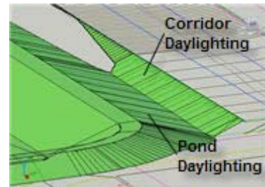
Figure 13. Unlike daylighting methods, grading projections can clean up on each other and provide easy solutions for complex designs.
